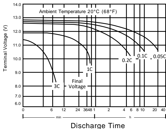
Discharge Characteristics
