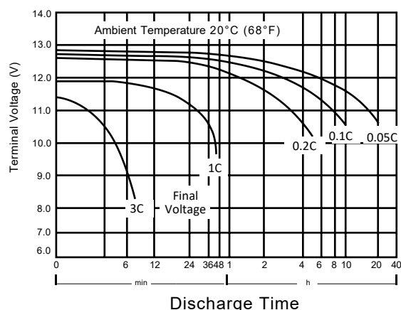
Discharge Characteristics
