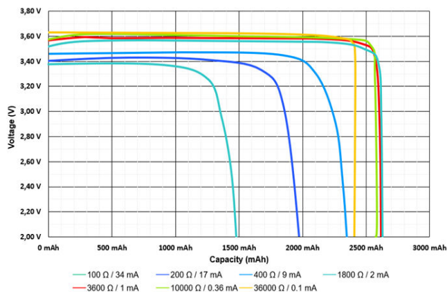
LS 14500 Typical discharge profiles at 20°C under various rates
